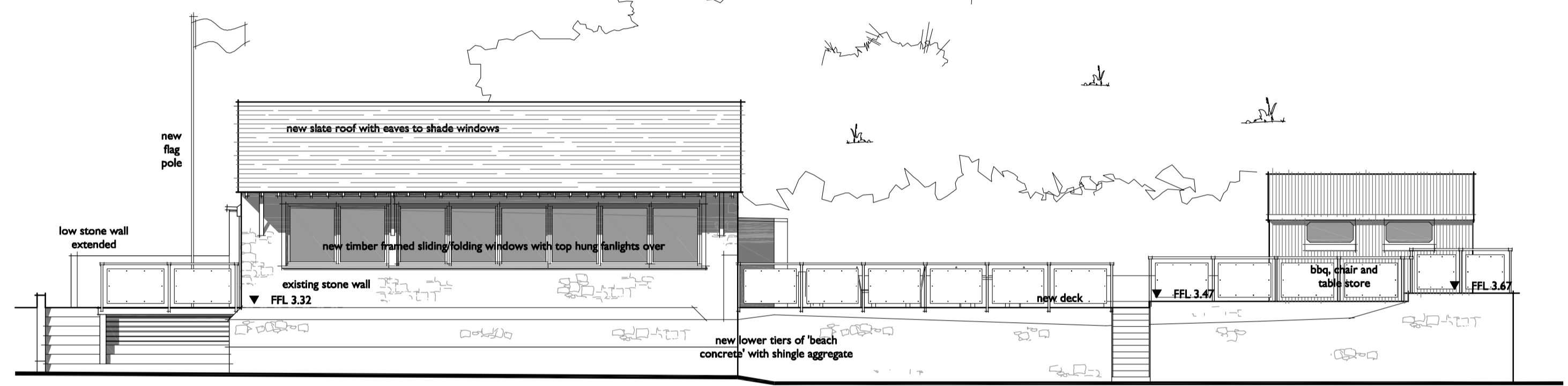
Beach Cafe and Shed - SE Elevation Beach Cafe and Shed - SE Elevation
