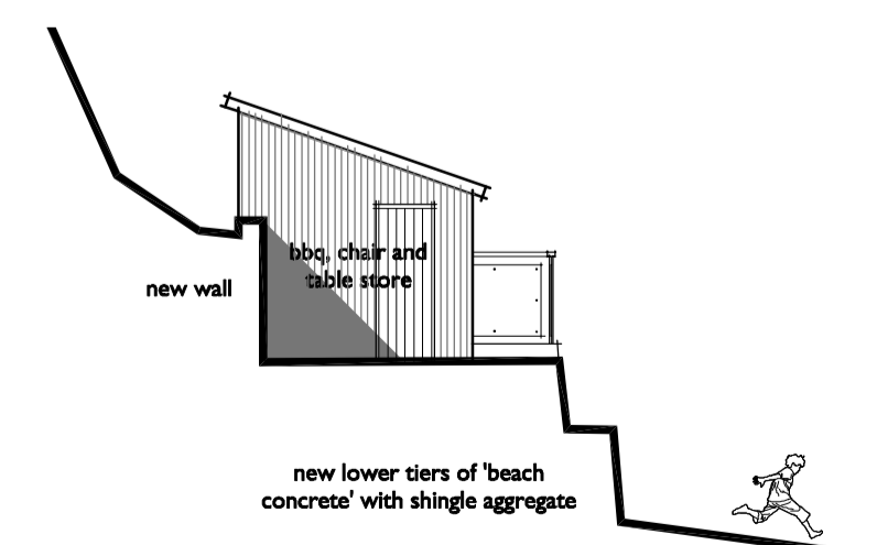
SW Elevation Shed
