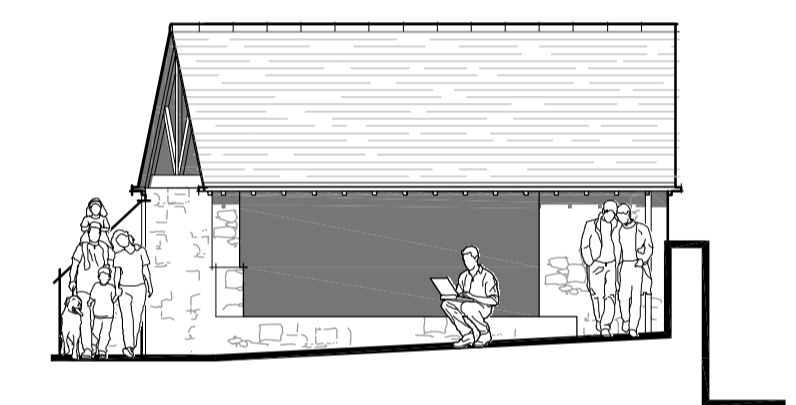
NW Elevation Shelter/Kiosk - NW Elevation
